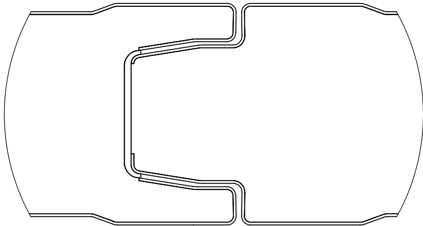
DETALLE JUNTA DEL PANEL / PANEL JOINT / JOINT DE PANNEAU ESCALA 1.5 : 1
