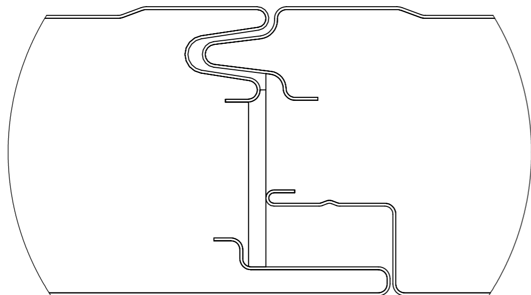
DETALLE JUNTA DEL PANEL / PANEL JOINT / JOINT DE PANNEAU ESCALA 1.5:1
